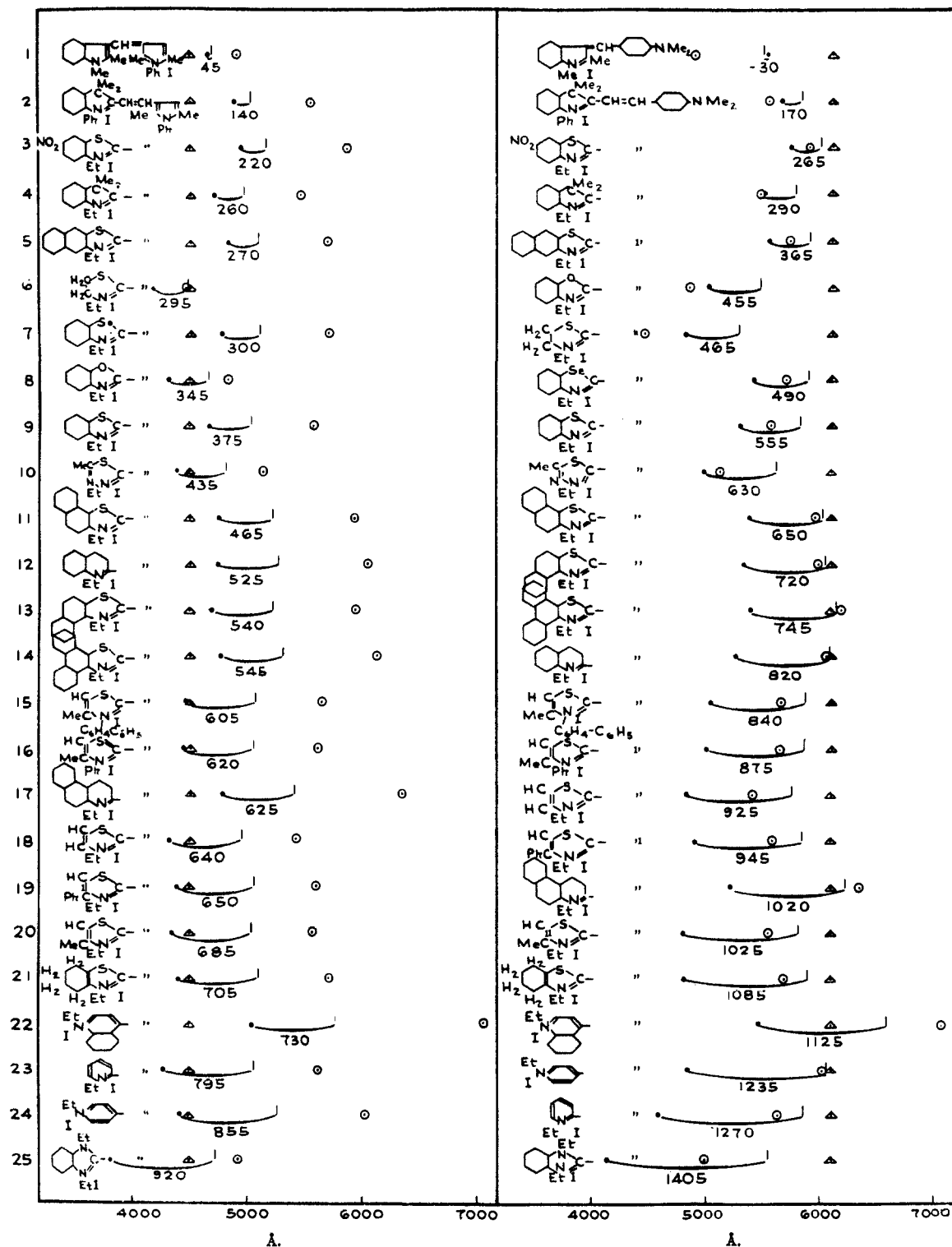
Fig. 1.—Order of basicity of twenty-five heterocyclic nuclei. Values of \lambda_{\max} in methyl alcohol are shown as follows: ● unsymmetrical cyanine; ▲ symmetrical cyanine with two pyrrole nuclei; ○ second symmetrical cyanine; | arithmetic mean between ▲ and ○; — indicates deviations, the magnitudes of which are given in Å.
