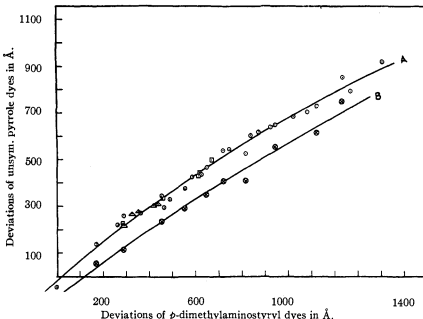
Fig. 6.—Relation between deviations in the p -dimethylaminostyryl and pyrrolo-carbocyanine series. Points \odot are obtained by plotting the deviations in Fig. 1 against those in Fig. 2, \Delta are points similarly obtained from Fig. 4 and \square are points obtained from Fig. 5; these points together give curve A. Points \odot are obtained by plotting deviations for the styryls against those of dyes containing the N -ethyl (or n -heptyl) 2,5-dimethylpyrrole nucleus. These give curve B.
